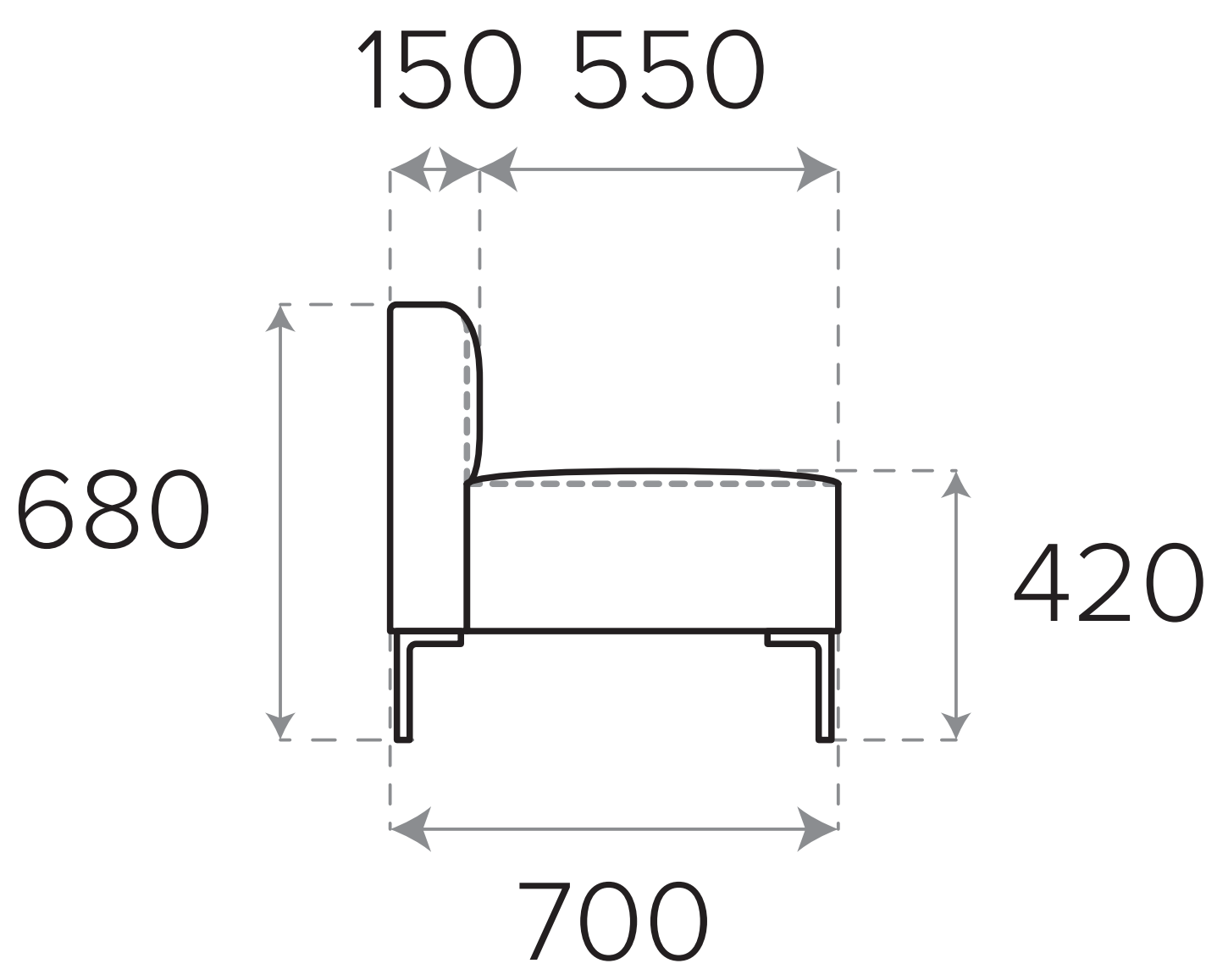
Genoa Modular Side Profile - with Back Elevation
