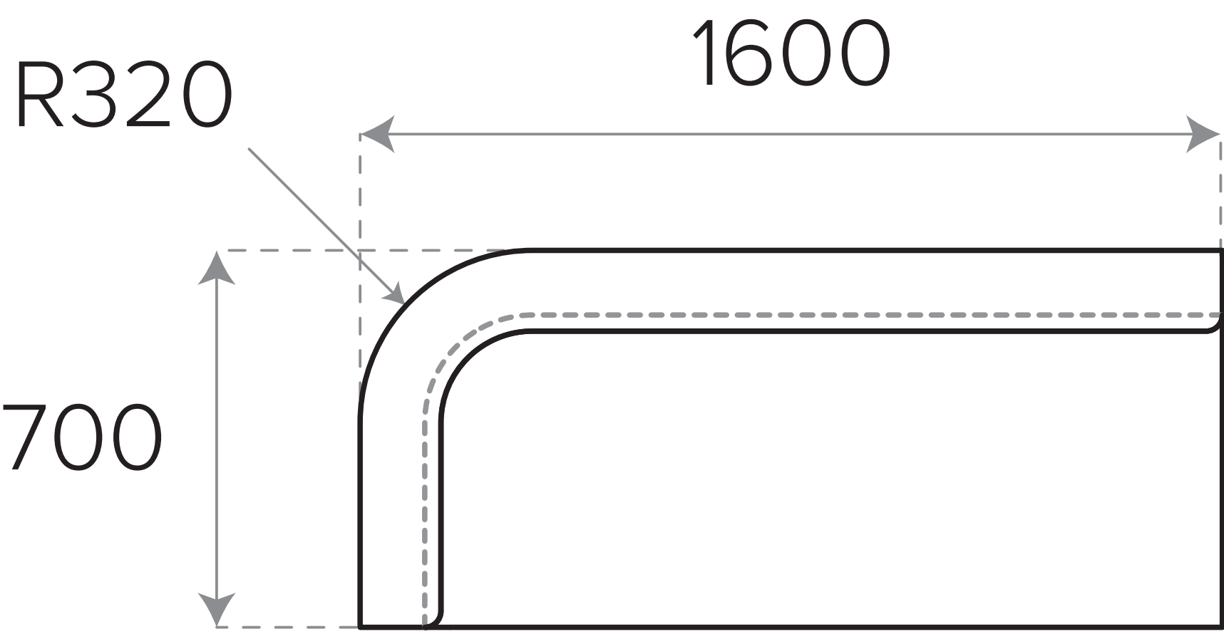
Genoa Modular 2 Seater 1A LHF Code: GMD2AL
