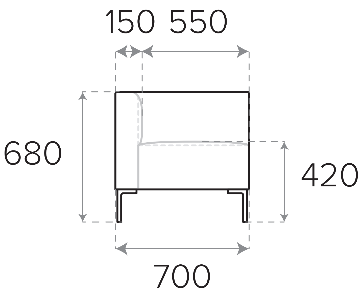
Genoa Sofa Side Profile Elevation
