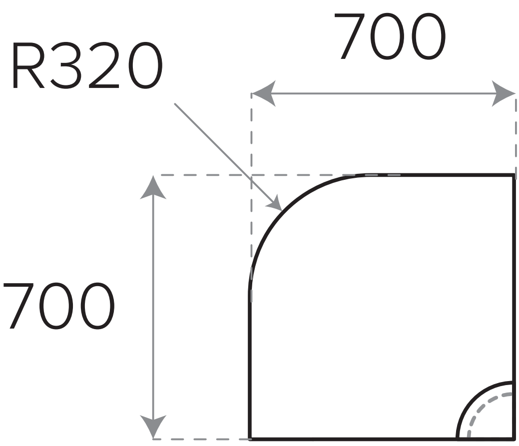
Genoa Modular Convex Corner Code: GMDVC
