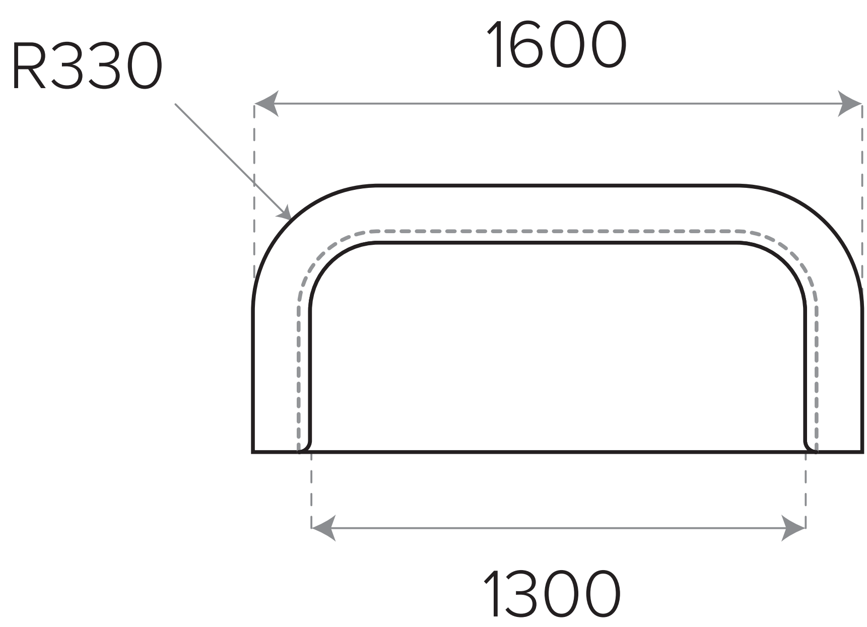
Genoa Sofa 2 Seater Code: GNC2
