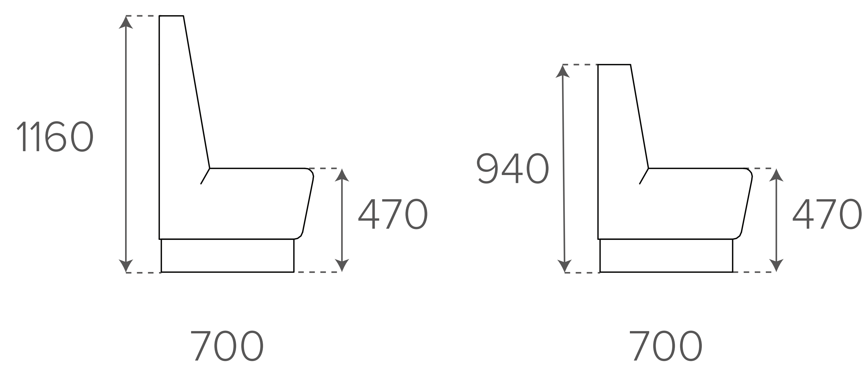
Aura Cafe Standard Heights Modular Side View
